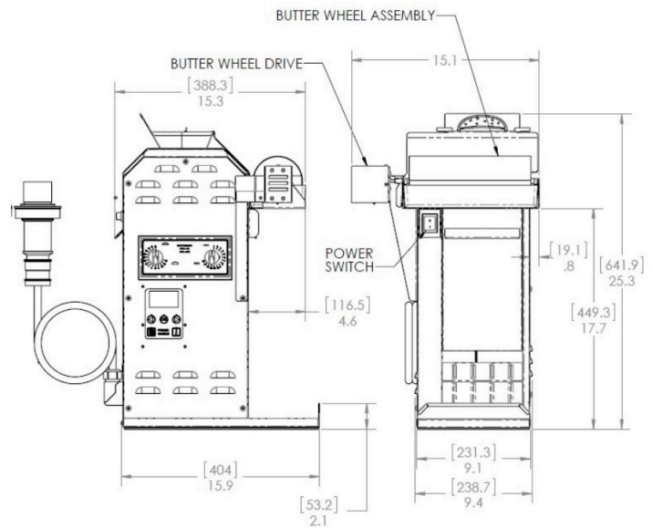
DCFT-ART-MCD Series With Butter Wheel
